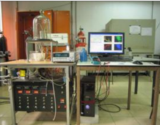
Gas sensing measurement system
