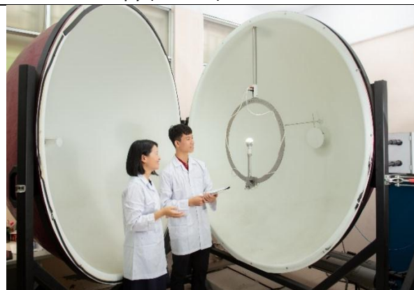
Integral Sphere
